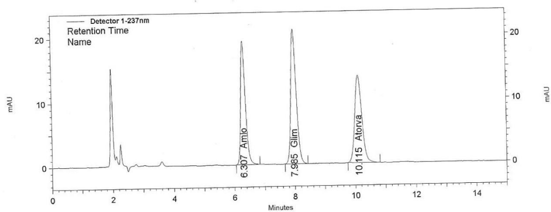
Figure 3.23. Chromatogram of amlodipine, glimepiride, and atorvastatin when setting the temperature at 28°C
